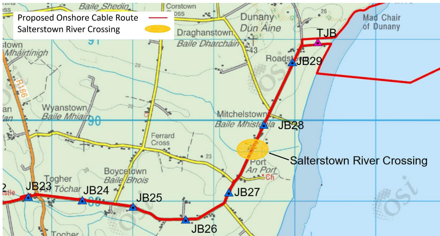
Figure 4: HDD location; Salterstown River Crossing
